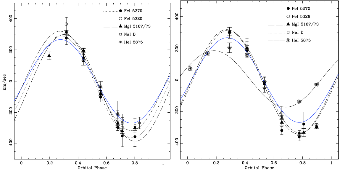
Fig. 7. Radial velocity measurements of the low ionization metal lines, (MgI and FeI) and the NaI and HeI emission lines. Left panel is for epoch 1 while the right panel is for epoch 2. Different symbols are for different emission lines and the notation is on the figure itself. Different line styles represent the best fit (as in Table 1) for the specified line. Note that not all best-fit radial velocity curves have been plotted for clarity. In both panels the blue solid line is the best fit determined for the H\beta emission in epoch 1.
