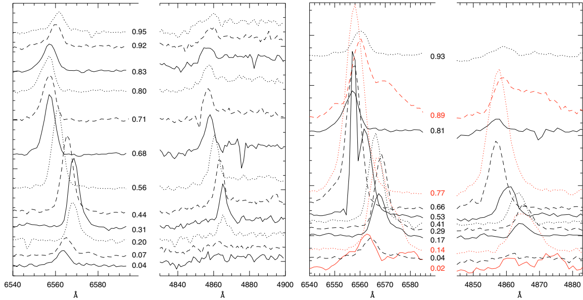
Fig. 3. Balmer emission line profiles for epoch 1 (left panel) and epoch 2 (right panel). Different line styles are just for clarity, while the lines in red color correspond to the four epoch 2 flaring/bursting spectra.
