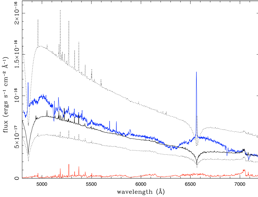
Fig. 8. Models vs. observation comparison. The black spectra are the three irradiation models (white dwarf + irradiated secondary star) described in Sect. 4. The dashed lines are for the LTE secondary atmosphere models, while the solid line is for the NLTE secondary atmosphere model. The top spectrum is for a 20 000 K white dwarf, while the two bottom ones are for a 11 900 K white dwarf. In blue color is the VV Pup epoch 1 faint phase spectrum. It is the average of the two spectra at phase 0.44 and 0.56 (see Fig. 2). We also show, in red color, the NLTE irradiated secondary atmosphere model alone. Flux units refer to the observed spectrum. The four models have been arbitrarily scaled. However, the NLTE irradiated secondary-star model (red) and the NLTE irradiated secondary-star model + the 11 900 K white dwarf (solid black) have been scaled by the same factor so that their relative flux and fractional contribution is preserved.
