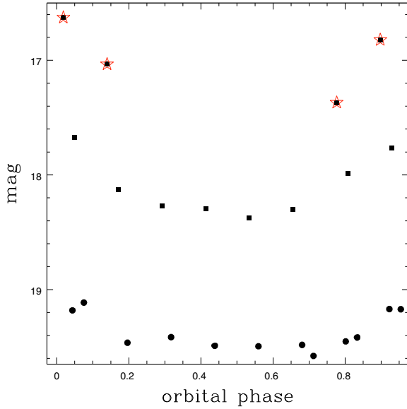
Fig. 1. Light curve extracted from the two data set by convolving each spectrum with a V -Johnson filter. Circles represent the data set of March 16. Squares represent the data set of March 22. Stars are for the last 4 frames in the March 22 data set which correspond to an increased mass transfer rate or to a flare episode.
