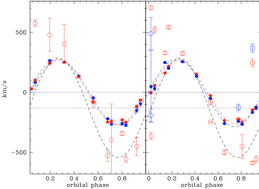
Fig. 4. Radial velocity measurements (left epoch 1, right epoch 2) of the Balmer lines H\alpha (red solid circles) and H\beta (blue solid circles) and their best fit (red and blue dashed lines). Open circles represent the secondary-satellite component (same color convention), while the dotted horizontal lines represent the \gamma velocity as determined by the sinusoidal fit. In black we report the best fit radial velocity curve determined by Howell et al. (2006a, sinusoidal dashed line) and its \gamma velocity (horizontal dotted line).
