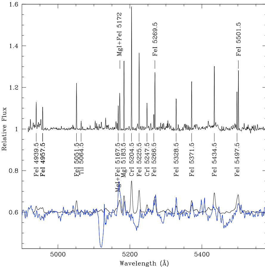
Fig. 9. Comparison of model and observation in the 4900–5600 Å region. In black color are the normalized model spectra at spectral resolution 0.5 Å (the resolution in the stellar atmosphere code, top ) and 5.0 Å (about the resolution of our optical spectra, bottom ). In blue color we plot the normalized faint phase spectrum of epoch 1, corresponding to the average of the two faint phase spectra at orbital phase 0.44 and 0.56. All the spectra have been normalized and shifted to a common reference wavelength. The observed blue spectrum and the low resolution model have been vertically shifted by the constant -0.4 for clarity.
