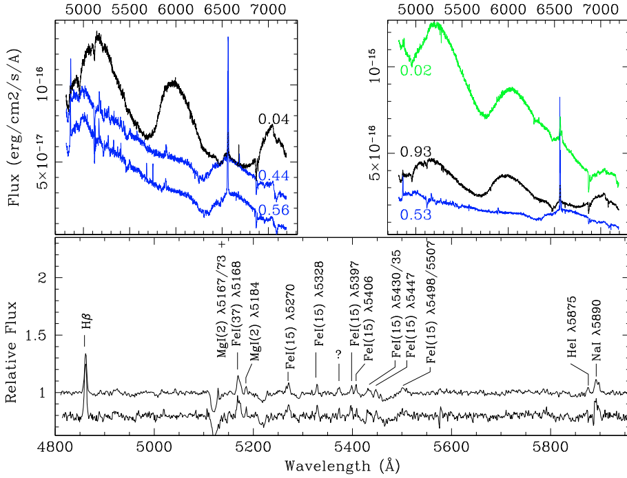
Fig. 2. Top panels: bright- (black) and faint- (blue) phase spectra of each data set, epoch 1 on the left and epoch 2 on the right. The numbers near each spectrum indicate their orbital phase. In the top left panel the spectrum at orbital phase 0.56 has been shifted vertically by the constant -0.2 \times 10^{-16} erg cm 2 s -1 . In the top right panel the green spectrum is the bright-phase spectrum observed during the accretion burst. Bottom panel: a zoomed-in view of the 4800–5960 Å region with the identification of the low ionization energy metal lines. The spectra in the bottom panel have been normalized. The top spectrum (in the bottom panels) is the average of the spectra at orbital phases 0.44 and 0.56 (properly shifted before co-addition) of epoch 1 data set; while the bottom spectrum is that at orbital phase 0.53 in epoch 2 data set. The bottom spectrum in the bottom panel has been vertically shifted by the constant -0.25 .
