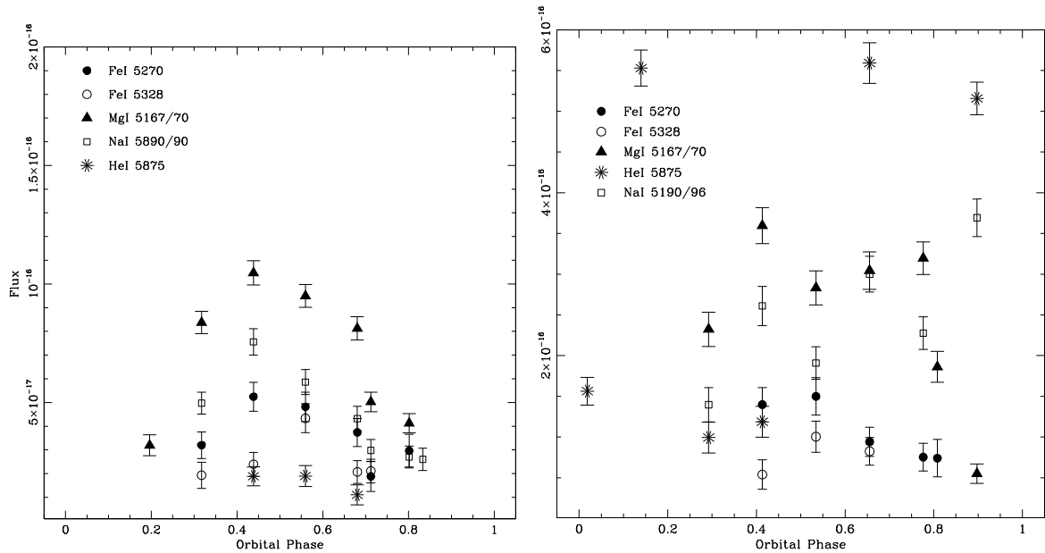
Fig. 6. Zoomed-in view of the emission line flux distribution versus orbital phase. The left and the right panels display the data of epoch 1 and 2, respectively. Different symbols are for different emission lines (notation on the figure itself). Note that in the case of the HeI emission the data point at orbital phase 0.78 has not been plotted for clarity, being a factor of two brighter than the brightest points displayed.
