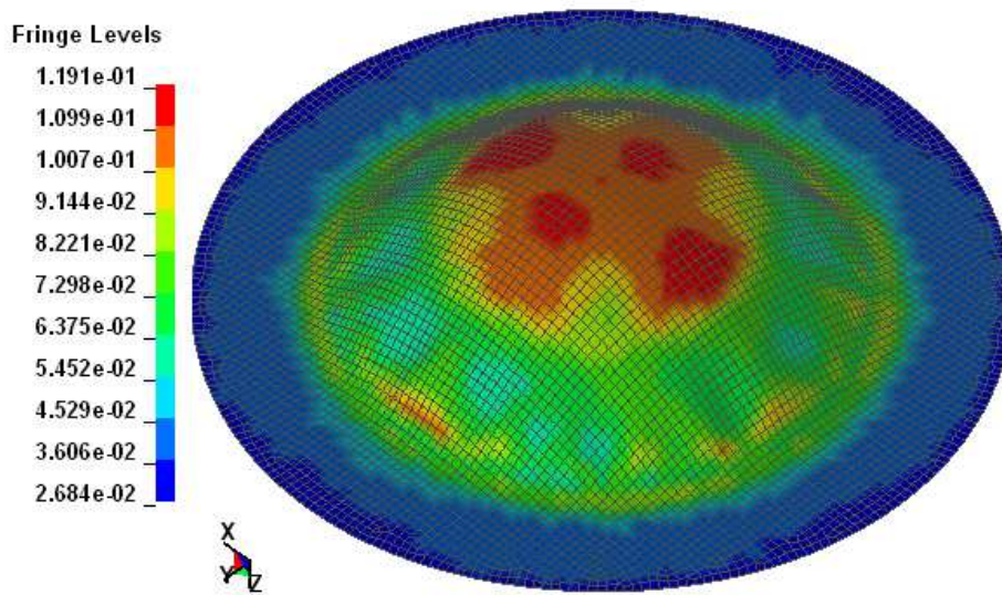
Figure5. Finite element results of FML-Curv of the major strain contours
