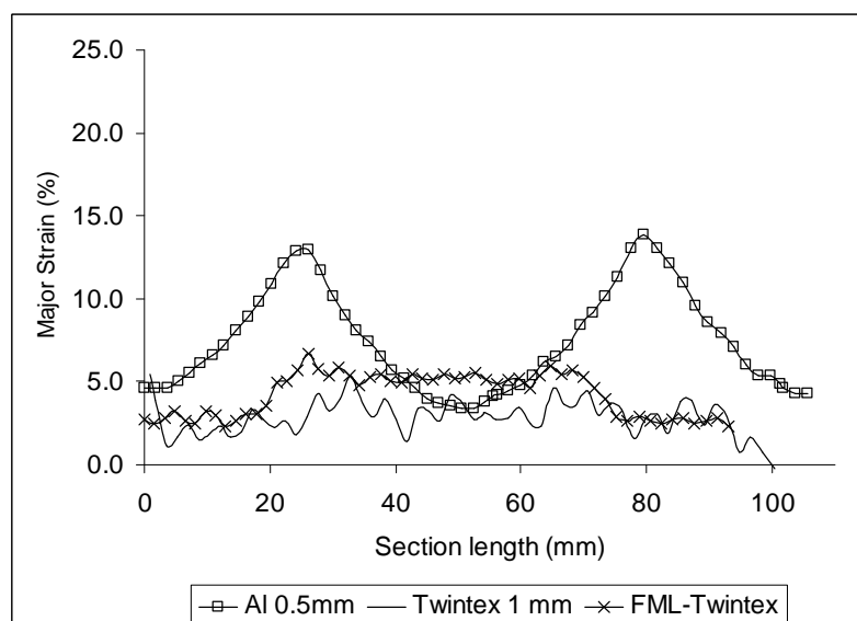
Figure4. Experimental results on meridian strains formed at room temperature to a depth of 25 mm
