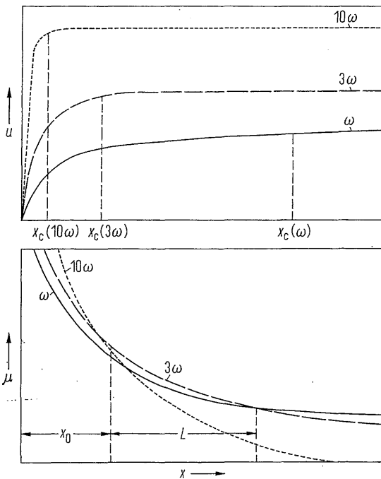
Fig. 3. Generalized behaviour of the wave velocity u and amplification factor \mu as functions of distance x , for the case of a Bickley jet emerging from a slit of infinitesimal width at x = 0 , for three different frequencies. The curves are based on the calculations reported by Drazin and Howard [6] and the coordinate x_c , given by eq. (19), shows the point of transition between the approximations (21) and (22) or (23) and (24). For the case of a jet of length L emerging from a slit of finite width at effective coordinate x_0 , the gain parameter G of eq. (25) is equal to the area under the appropriate \mu curve between x_0 and x_0 + L .
