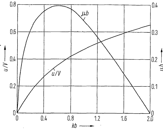
Fig. 2. The wave velocity u = V c_r and the amplification factor \mu = k c_i / c_r as functions of the frequency parameter kb for a jet of Bickley profile, as deduced from the calculations reported by Drazin and Howard [6]. V is the centre velocity of the jet, b the width parameter, and k = \omega/u where \omega is the angular frequency. In terms of the original analysis, c_r is the real part and c_i the imaginary part of the normalized wave velocity u/V and kb = \alpha .
