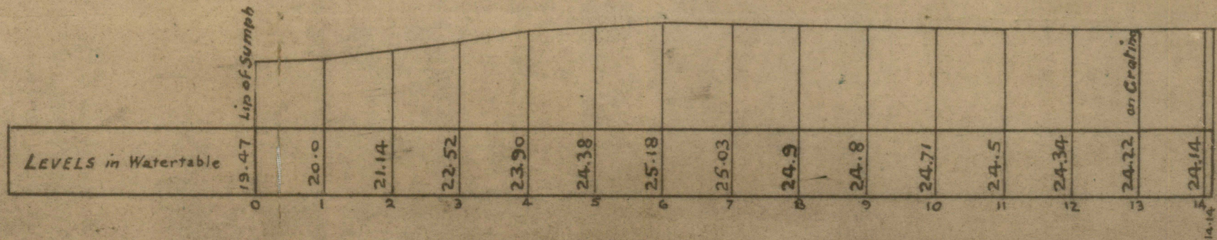
SECTION Scale Horizontal 2 chains, Vertical 20 feet to an inch
