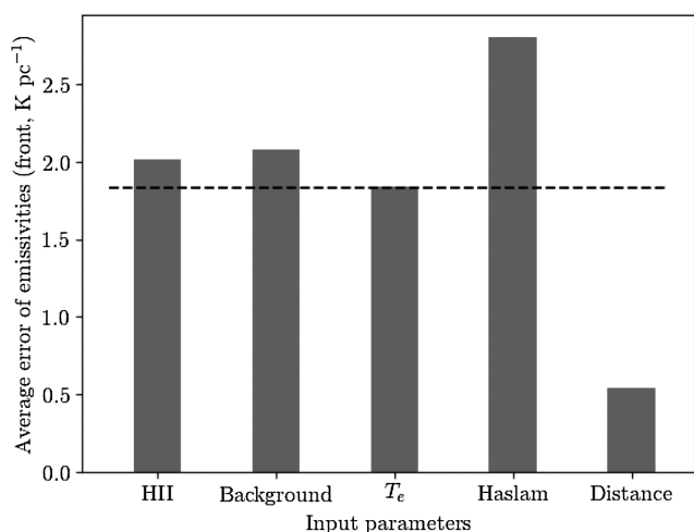
Figure 7. The contribution of different input parameters to the error of the emissivities at 76.2 MHz from \text{H II} regions to the Sun. The total error of the emissivity is from different input parameters which are the rms of the absorbed region ( \text{H II} ), the rms of the nearby region (background), the error of the electron temperature ( T_e ), the rms of the background region in the Haslam map (Haslam), and the error of the distance from \text{H II} region to us (distance). Each error here is an average of all the 152 absorption measurements. ‘Front’ on the y-axis means the emissivities are averaged along the path from \text{H II} region to the Sun (in front of \text{H II} region). The error from the rms of the Haslam map contributes the most to the final error of the derived emissivities. The horizontal line indicates the average uncertainties of all the derived emissivities between the \text{H II} region and the Sun. Note that the error involved in scaling the Haslam map to our frequencies is not included here.
