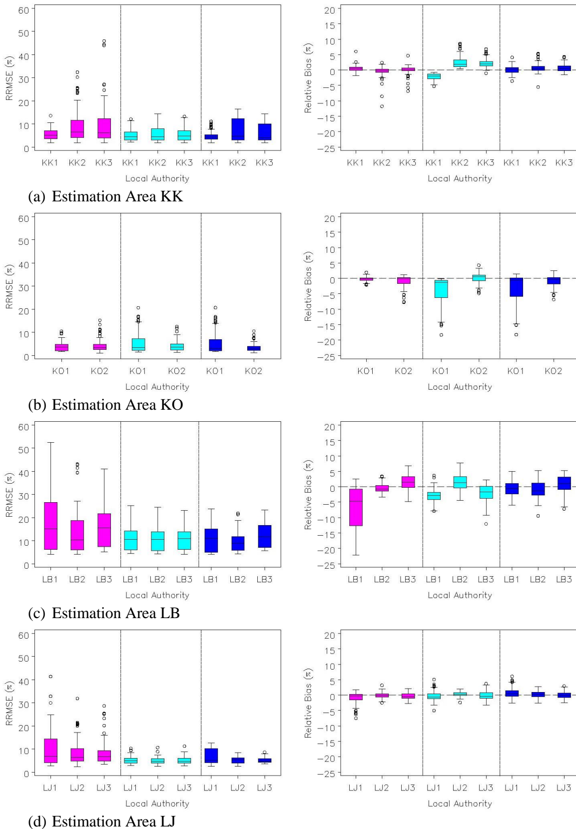
Figure 1. Boxplots showing the RB and RMSE distribution of the different small area estimators for the selected four estimation areas. For each plot the left panel represents the direct estimator, middle panel represents the synthetic estimator, and the right panel represents the local fixed effects model.
