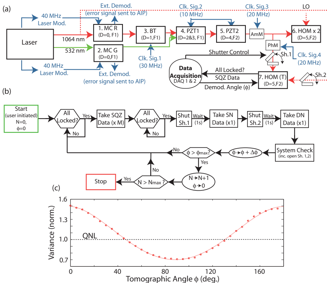
FIG. 5. (Color online) (a) Experimental setup. MC – mode cleaner (R – red, G – green); BT – bow-tie cavity; PZT – piezo-transducer phase lock; HOM – homodyne lock (T – tomographic, x 2 – double homodyne); AmM – amplitude modulator; PhM – phase modulator; Sh – mechanical shutter; SQZ data – squeezing data; D – lock dependencies (0 = no dependencies); F – FPGA lock is controlled from; Ext. Demod. – external demodulation carried out for these locks to produce the error signal; AIP – analog input; DAQ – data acquisition card; Clk. Sig. – clock signal; and LO – local oscillator. (b) Flow diagram of data acquisition procedure used to take squeezing data (SQZ) for various angles of the tomographic lock \phi , as well as take dark noise (DN) and shot noise (SN) traces. Values for the number of experimental runs N , number of squeezing traces for each tomographic angle M , and change in tomographic lock angle between runs \Delta\phi are defined by the user. (c) Plot of variance in noise normalised to the quantum noise limit (QNL), as a function of tomographic lock angle taken using the above procedure with a total of 1.2 million points per angle, and \Delta\phi = \pi/36 . Circles: data points; dashed line: theoretical fit.
