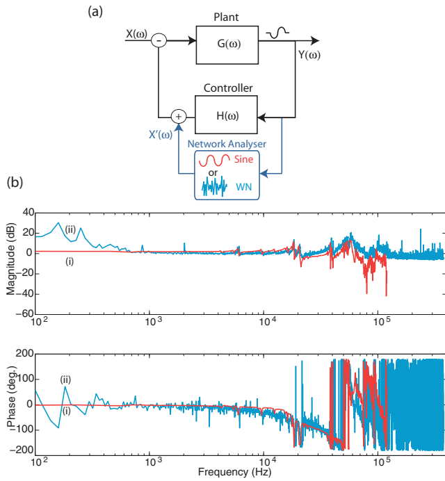
FIG. 1. (Color online) (a) Block diagram of a basic feedback control system. Here G(\omega) and H(\omega) are the transfer functions of the plant and controller respectively, with X(\omega) being the input noise and Y(\omega) being the output of the system (i.e., error signal). Also shown is the placement of a network analyzer, with X'(\omega) being the extra noise added to the system in the form of a swept sine wave (Sine) or white noise (WN). (b) Bode plot of the transfer function of a code-cleaner cavity for (i) a network analyzer (model MS4630B from Anritsu) and (ii) a white noise generator included in the code.
