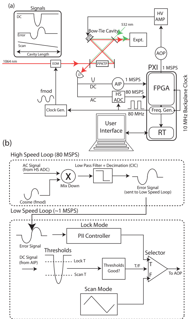
FIG. 2. (Color online) (a) Depiction of the physical system and hardware required for digital locking using the code presented here, in this case for a bow-tie OPO cavity doubly resonant with a green (532 nm - dashed line) and a red (1064 nm - solid line) field, the latter being used to lock the cavity position on reflection. MSPS – M samples s^{-1} ; PXI – PXI chassis; FPGA – field programmable gate array card; Freq. Gen. – frequency generator; RT – real time controller; AIP – analog input to FPGA (sampling frequency < 1 MSPS); HS ADC – high speed analog to digital converter (80 MSPS); D – detector; Clock Gen. – digital clock generation board; f_{mod} – modulation frequency for lock; EOM – electro-optic modulator; PZT – piezo-electric transducer; PPKTP – periodically poled potassium titanyl phosphate crystal; HV Amp – high voltage amplifier; and Expt. – rest of experiment. Inset shows the different signals which are used for locking (DC – dc reflection signal; ES – Error signal; Scan – scan function) as a function of PZT position. (b) Depiction of LabVIEW® code used to program FPGA cards. CIC – cascaded-integrator-comb filter; PII controller – proportional, integral, double integral controller; Scan T – scan threshold; Lock T – lock threshold; T – true; F – false.
