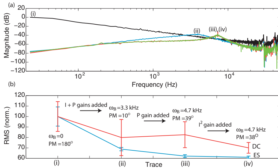
FIG. 3. (Color online) (a) Magnitude plot of system transfer function for an OPO cavity with controller gain increasing from (i) to (iv). (b) Normalised rms values for these traces for both the error and dc signals. Error bars show standard deviation across 10 runs used for each point. Also shown is the sequence in which the different gains are added, the bandwidth of the system ( \omega_B ) and phase margin (PM) measured by the code.
