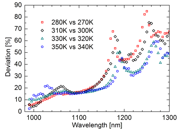
FIG. 9. Relative increment of the absorption coefficient for every 10 K increment around RT.
