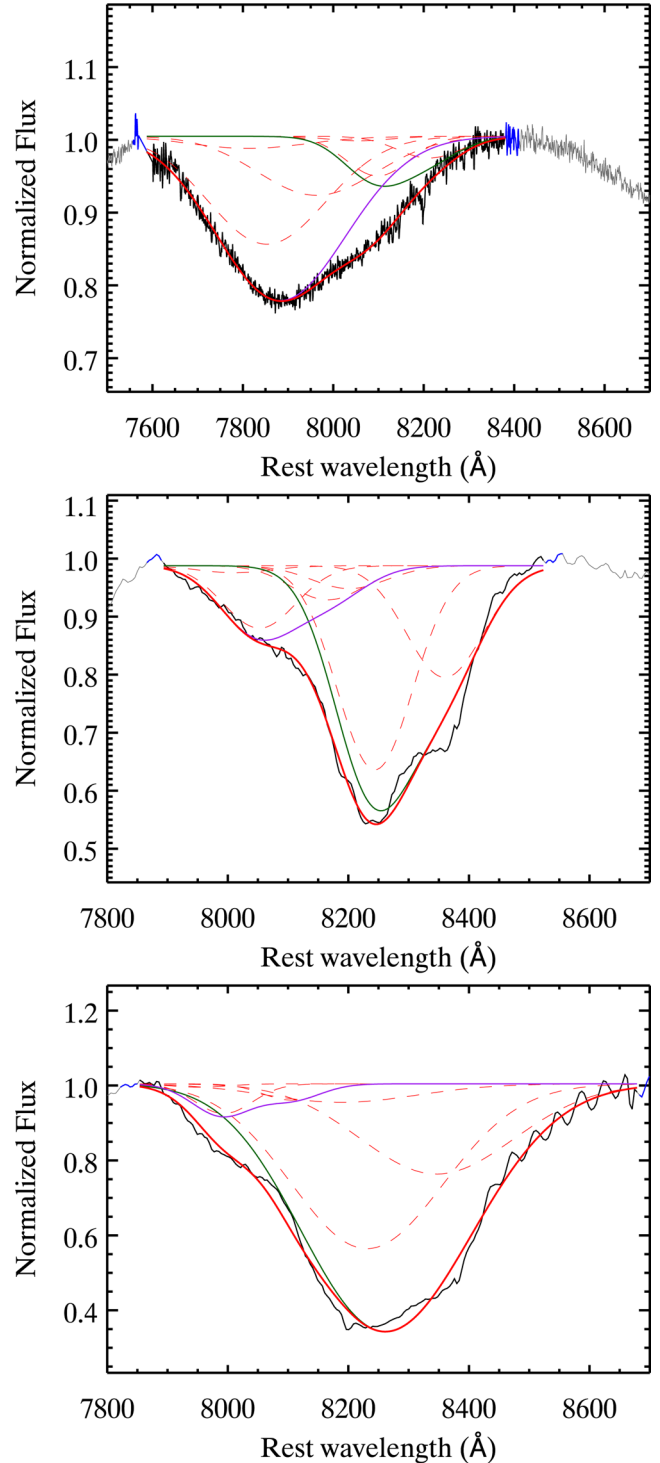
Figure 8. From top to bottom: the \text{Ca II} NIR absorption at -16, +5 , and +15 d, respectively. The black curve shows the range we fit the line profile. The blue continuum regions near the left and right side of the line profile are the regions we select to fit the pseudo-continuum. The red solid line is the best fit to the line profile, which is the superposition of all the line components used for the fitting (represented as dashed lines). The green curve represents the superposition of all the components in \text{Ca II} NIR PVF. The purple curve represents the superposition of all the components in the \text{Ca II} NIR HVF.
