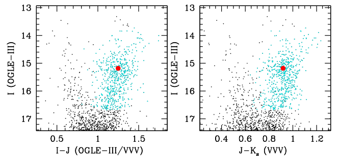
Figure 10. CMDs in I versus (I - J, J - K_s) towards (l, b) = (1^\circ 68, -3^\circ 58) . Symbols are as in Fig. 2. This sightline, with an anomalous large extinction coefficient of E(J - K_s)/E(I - J) = 0.66 , gives no indication from its CMD of being the product of a systematic such as differential reddening.
