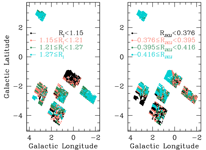
Figure 9. Spatial distribution as a function of Galactic coordinates (degrees) of the optical extinction coefficient R_I = A_I/E(V - I) (left-hand panel) and the near-IR extinction coefficient R_{JKIJ} = E(J - K_s)/E(I - J) (right-hand panel). The colours denote quartiles weighted to have approximately equal surface area. Though both the optical and near-IR extinction coefficients have significant variations across the sky, these variations are uncorrelated.
