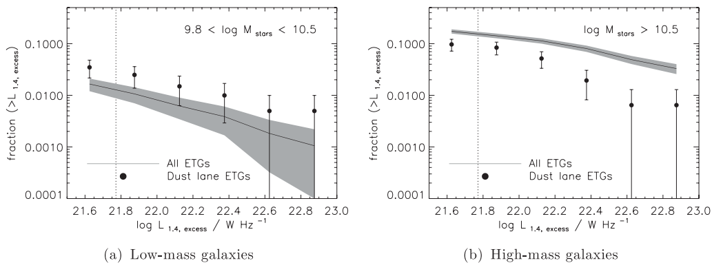
Figure 4. Left: cumulative fractional RLFs for low-mass dust lane (points) and a matched sample of low-mass early-type galaxies (shaded region) with 0.01 < z < 0.05 . Standard V/V_{\text{max}} corrections are applied. The dashed line corresponds to the completeness limit at the back of the volume. Right: same as the left-hand panel but for massive galaxies. Massive dust lane early types host significantly fewer radio AGN than the control sample.
