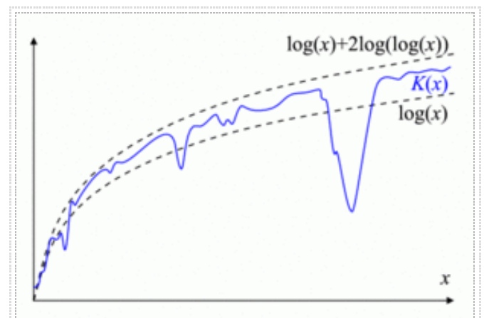
Figure 1: Schematic graph of prefix Kolmogorov complexity K(x) with string x interpreted as integer. K(x) \geq \log x for "most" x and K(x) \leq \log x + 2 \log \log x + c for all x for suitable constant c .
