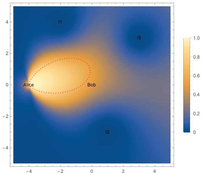
Fig. 15. Secrecy pressure outage map of the surface S . Eve's distribution is Gaussian and centered in three different positions: at Alice's, at Bob's and at the first interferer's I_1 .
