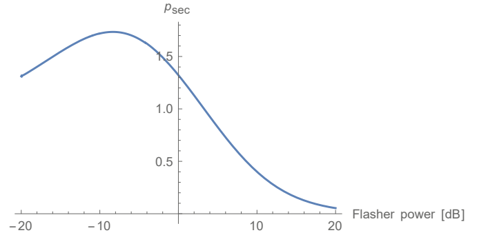
(b) Secrecy pressure as a function of the power of the additional interfering node (flasher). The flasher is supposed to be placed in the center of the lighter zone depicted in Fig. 8(a).
