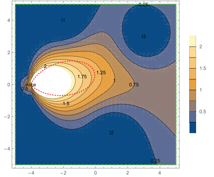
(a) Map of the secrecy pressure as a function of Bob's position. Eve can be everywhere over the surface.
