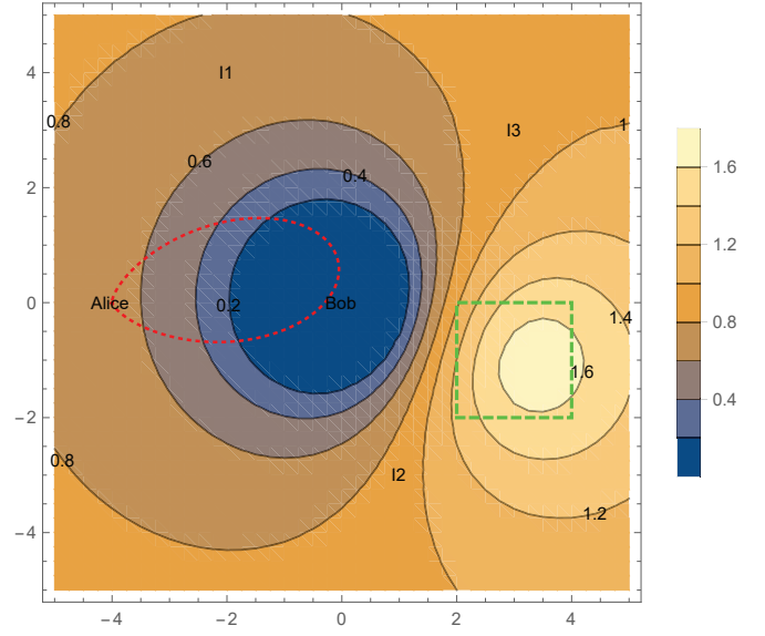
(a) Secrecy map over the surface S when the optimization problem is solved respect to the position of the additional interfering node (flasher). Eve is supposed to be somewhere in the green dotted line.
