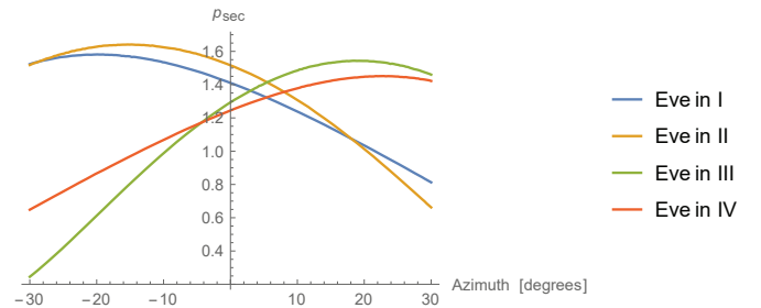
Fig. 6. Secrecy map for different positions of Eve (I, II, III and IV quadrant) when the optimization problem is solved respect to Alice's antenna orientation.
