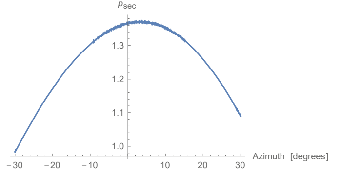
Fig. 5. Secrecy pressure when the optimization problem is solved respect to Alice's antenna orientation.
