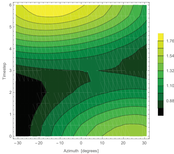
Fig. 13. Eve's mobility: scenario description and secrecy map over azimuth of Alice's antenna.
