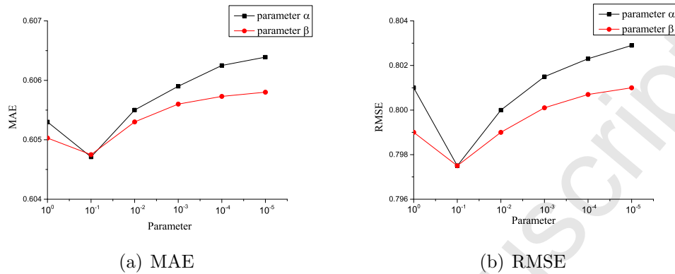
Figure 4: Impact of parameter \alpha and \beta in FilmTrust
