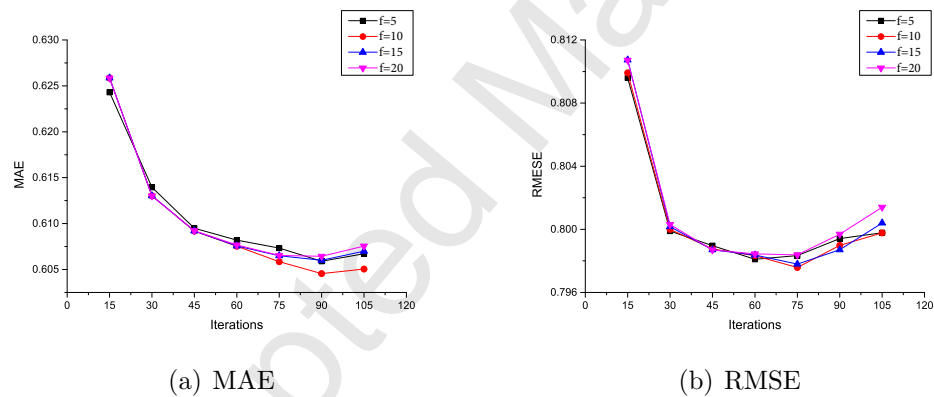
Figure 5: Performance on FilmTrust with different value of f
