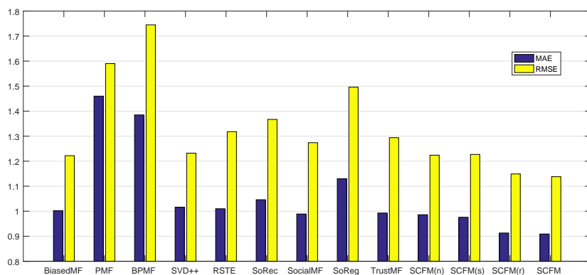
Figure 2: Baseline Algorithm Comparison III
