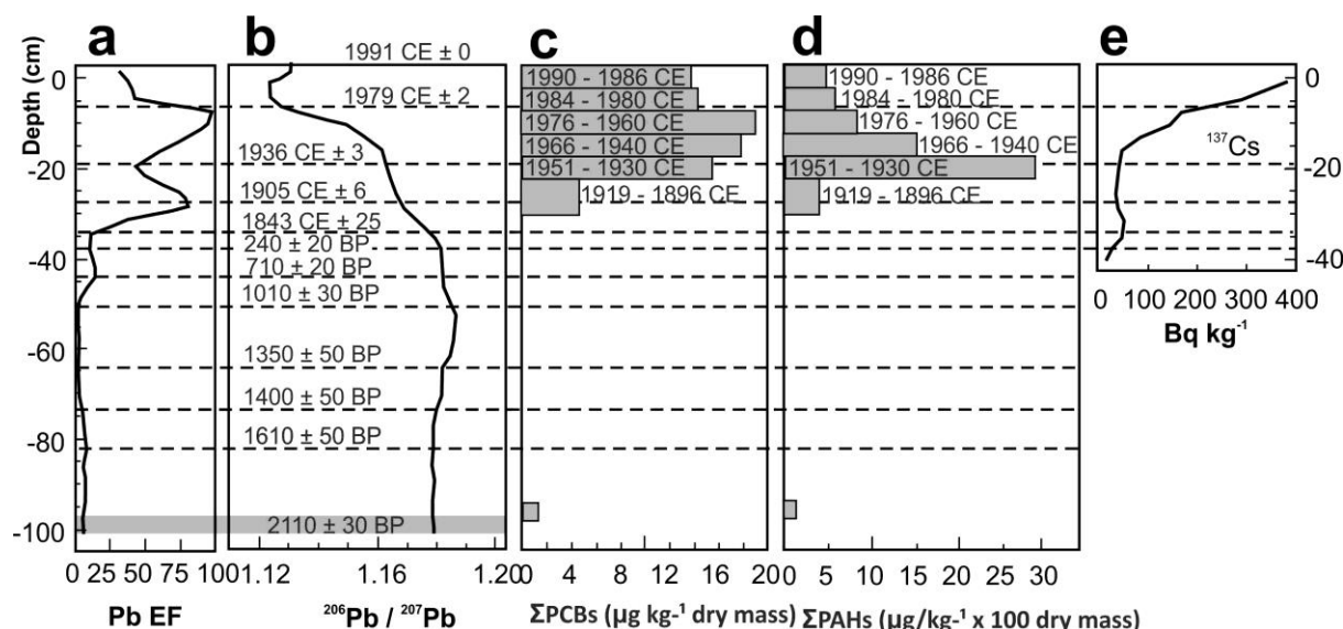
Figure 21. Core from Etang de la Gruère, Switzerland, collected in 1991 CE: a) Pb Enrichment Factor (EF) calculated as the ratio of Pb/Sc in the peats, normalized to the background value (from Shotyk et al. 1998); b) Pb isotopic values (from Shotyk et al. 1998); c) \Sigma PCBs (from Berset et al. 2001); d) \Sigma PAHs (from Berset et al. 2001); e) ^{137}\text{Cs} (from Appleby et al. 1997). Succession dated using ^{210}\text{Pb} to 35 cm depth (Appleby et al. 1997) and ^{14}\text{C} yr BP from 35 cm to base (Shotyk et al. 1998).
