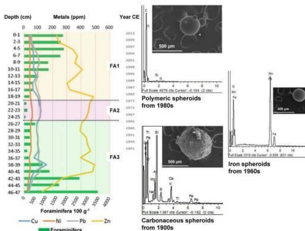
Figure 10. Metal concentrations (Cu, Ni, Pb, Zn) versus foraminiferal density in the Urola estuary (northern Spain). FA1–FA3 represent three distinct foraminiferal assemblages referred to in the text. Modified from Goffard (2016).
