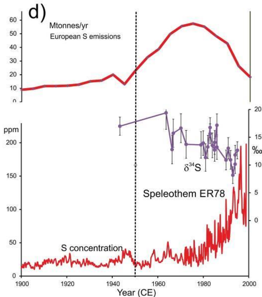
Figure 29. Ernesto Cave, Italy: a) Age model based on lamina counting related to local mean air temperature (Frisia et al. 2003); b) \delta^{18}\text{O} and \delta^{13}\text{C} profiles (Scholz et al. 2012); c) Radiocarbon profile and comparable European atmospheric emissions (Fohlmeister et al. 2011); d) S concentration and \delta^{34}\text{S} (Frisia et al. 2005, Wynn et al. 2010).
