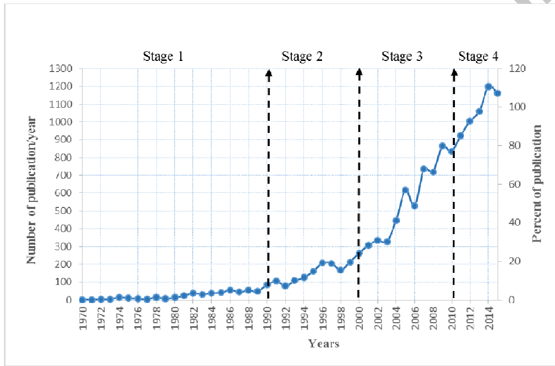
Figure 3: Publishing trend in the area of integrated water assessment and modelling
