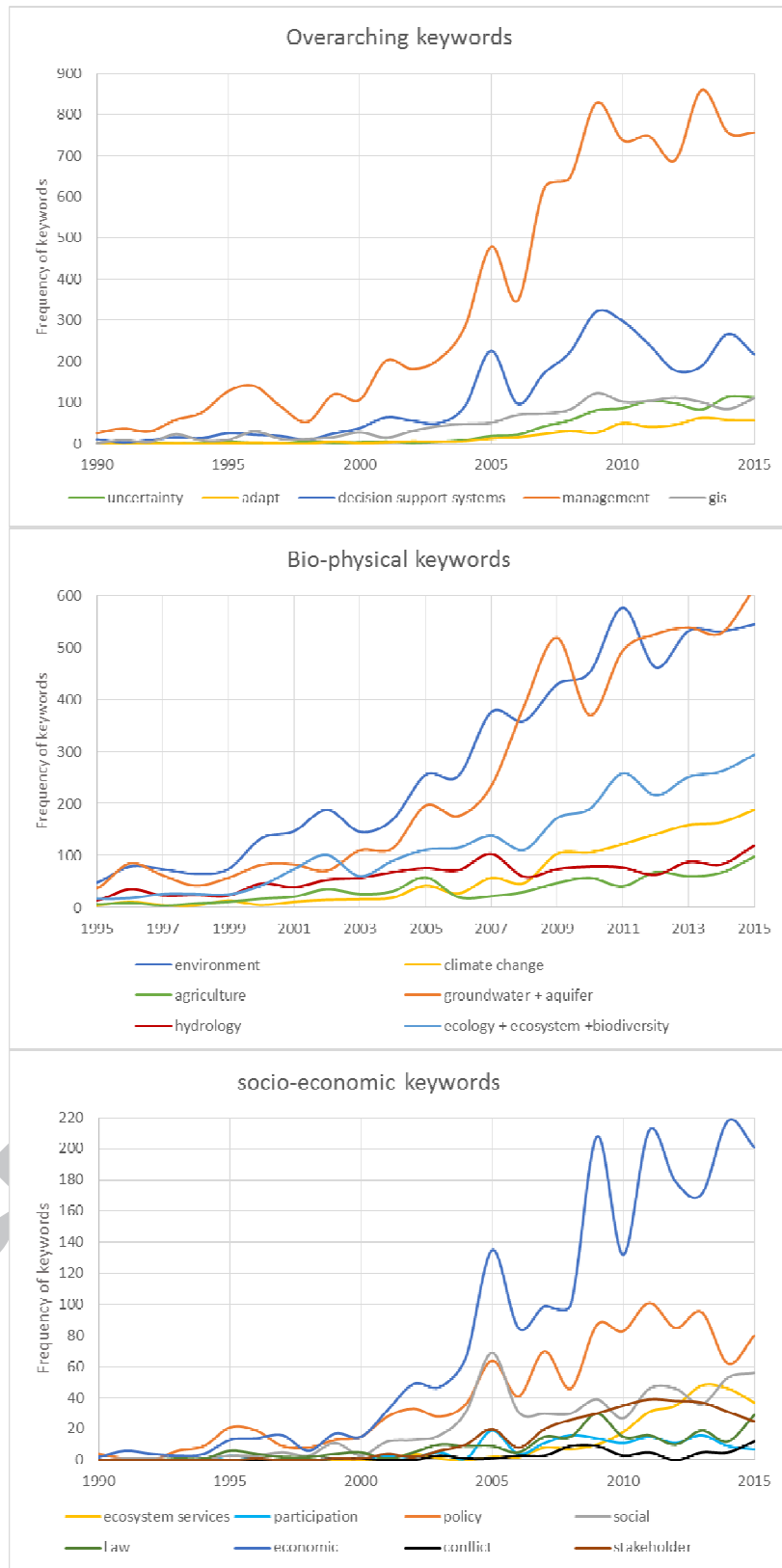
Figure 11 (a, b, c): Trends of the keywords in the overarching, bio-physical, and socio-economic categories
