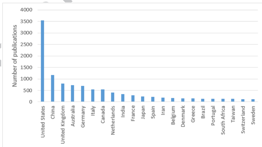
Figure 6: Number of publications for countries with over 100 journal papers on IWAM
