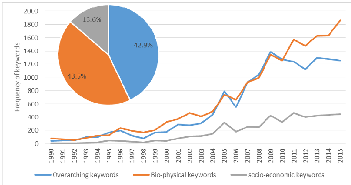
Figure 10: Keyword category trend and overall percentage
