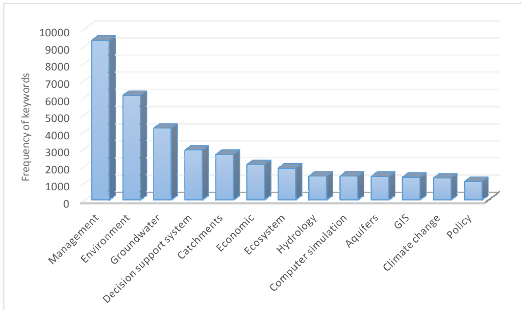
Figure 7: Frequency of popular keywords listed in IWAM articles
