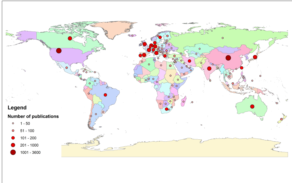
Figure 5: Map of the distribution of IWAM articles published by country
