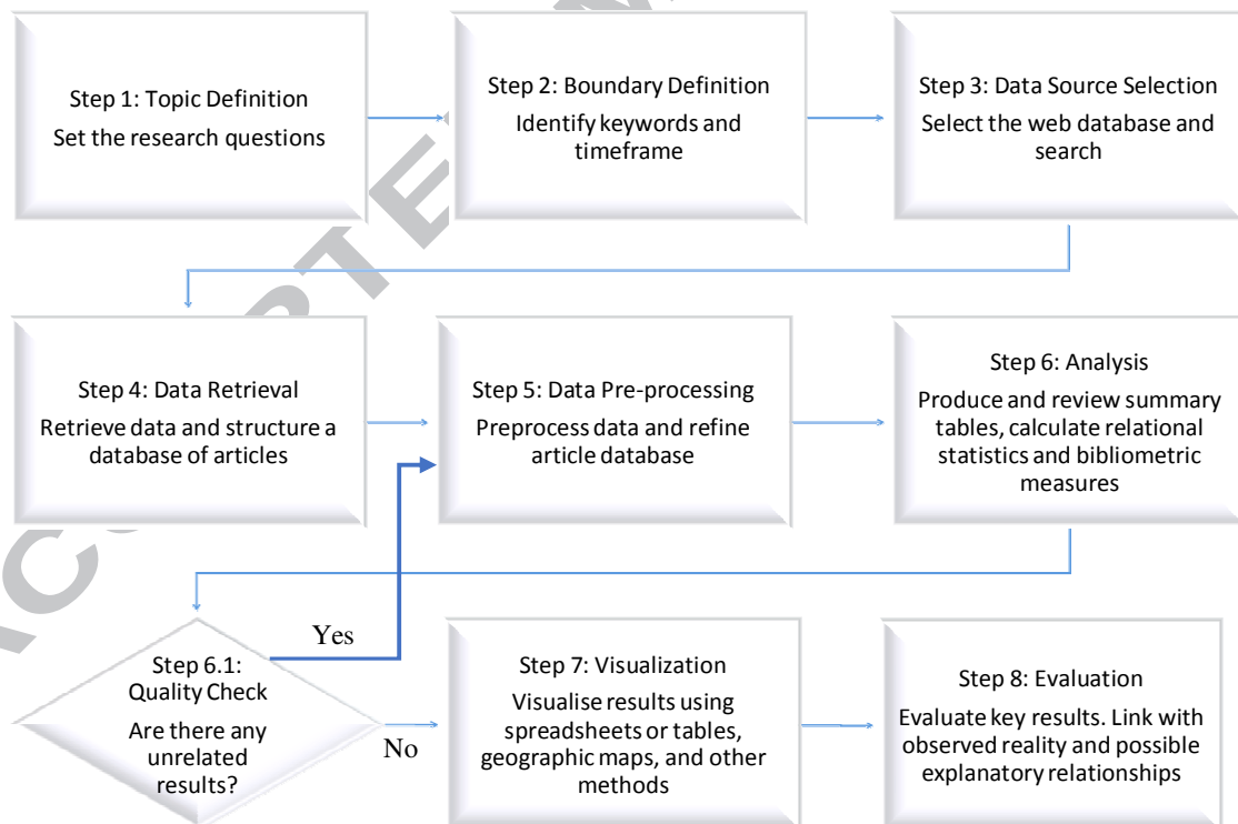
Figure 1: The stepwise approach to bibliometric analysis applied in this study. Each step is conducted in sequence with a feedback between step 6.1 and 5 occurring if the results are to be checked.
