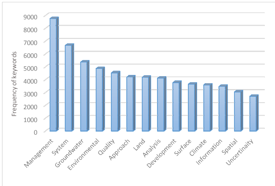
Figure 9: The most common key terms in IWAM abstracts
