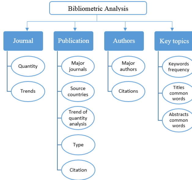
Figure 2: A concept map of the elements under investigation in the bibliometric analysis
