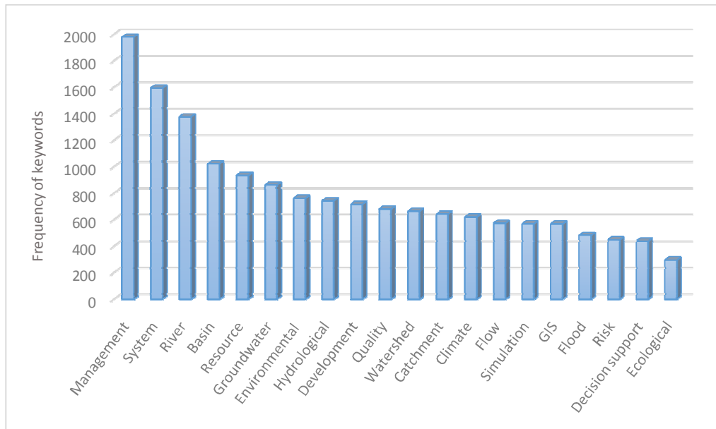
Figure 8: The most frequent title words in IWAM articles
