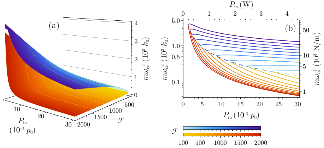
Figure 11.3: Comparison of the optical stiffness obtained with single- and a multi-mode inputs. The axes are scaled in terms of the constants p_0 and k_0 introduced before. Physical scaling in SI units is also given, corresponding to \lambda = 1064 \text{ nm} , \omega_{\text{FSR}} = 2\pi \times 750 \text{ MHz} , and m = 1 \text{ mg} . (a) Full comparison as a function of input power P_{\text{in}} and cavity finesse \mathcal{F} . The blue surface is the spring constant obtained from a single-mode input. The red surface is the minimum spring constant achievable when a multi-mode continuous ramp input is used instead. (b) Cross sections of the full comparison for different values of finesse. The starting point of each curve corresponds to the lowest power satisfying the trap depth requirement at a specific finesse, i.e. such that the cavity power is at least 1.5p_0 and the corresponding force is at least 1.5f_0 . The locus of such points is shown as a dashed line. A further increase in power shifts the balancing point f_0 along the profile of the Lorentzian force function, yielding different optical stiffness. Each point on a red curve corresponds to the lowest stiffness achievable, which is obtained when the maximum cavity power is kept constant at 1.5p_0 to satisfy the trap depth requirement while the additional power available is used to make the ramp wider.
