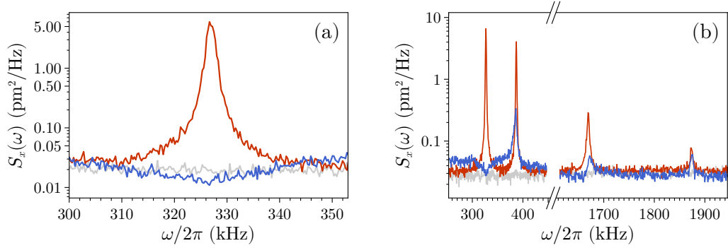
Figure 6.4: Displacement spectra of a nanowire subject to feedback cooling. The nanowire is \approx 60\,\mu\text{m} in length, \approx 220\,\text{nm} in diameter, gold-coated, and in vacuum. (a) Single-mode cooling. The amplitude of the thermal fluctuations (red) is suppressed down to the level of the background noise and beyond (blue), giving rise to squashing in the displacement spectrum. The grey trace indicates the detection noise in the absence of the nanowire. (b) Multi-mode cooling. The parameters of the feedback are optimized towards cooling of the mode with the lowest frequency, although in order to obtain cooling of the higher-order modes the phase of the feedback cannot be adjusted optimally and more measurement noise is injected into the system.
