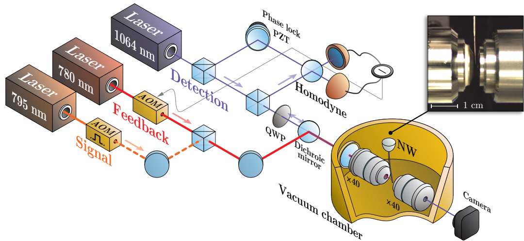
Figure 4.4: Comprehensive scheme of the experiment on the nanowire (NW). The three optical branches are used for the detection of the thermal motion of the nanowire (1064 nm), for the continuous or periodic feedback to suppress the thermal fluctuations (780 nm), and for the application of an impulsive signal during periods of feedback quiescence (795 nm). The inset shows a close-up photograph of the tungsten needle with the nanowire at its tip between the microscope objective lenses.
