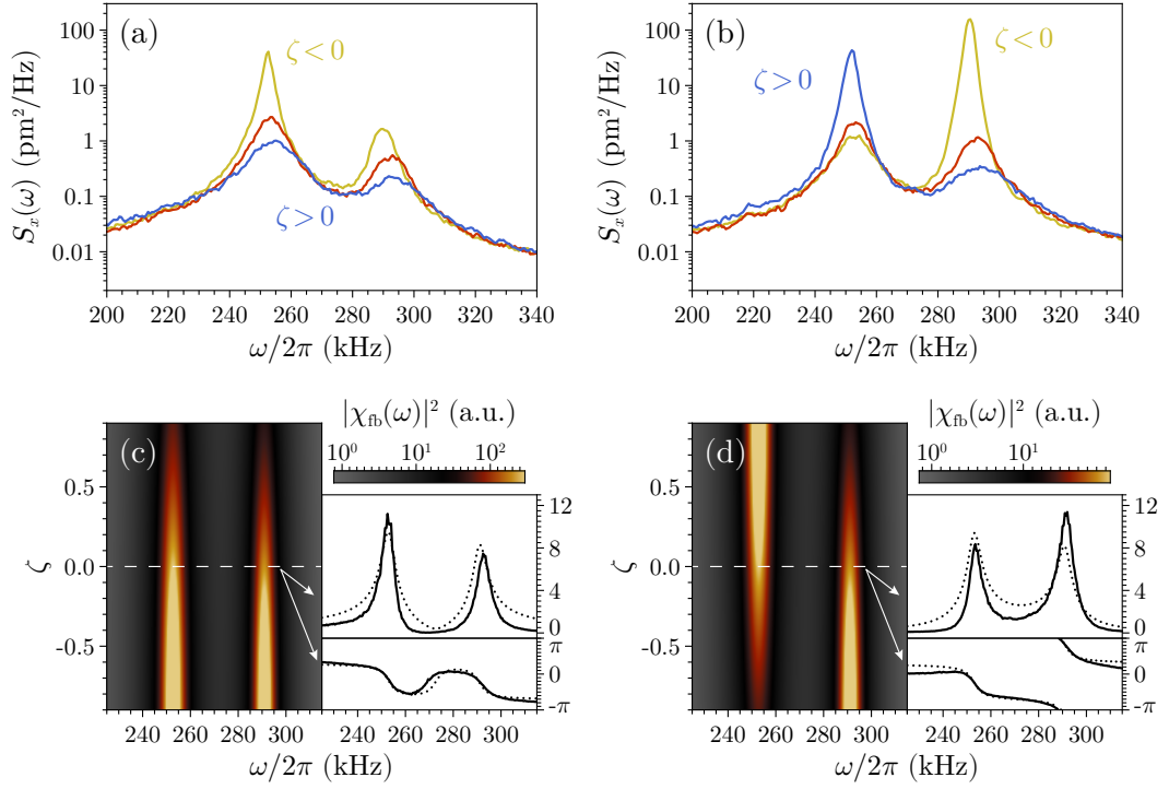
Figure 6.3: Response to feedback of a nanowire at different orientations. The nanowire is gold-coated, \approx 50\ \mu\text{m} in length and \approx 300\ \text{nm} in diameter, and it is always oriented at about 45^\circ with the incident beam in order to detect the two spatially orthogonal modes together. (a–b) Displacement spectra in normal conditions (red) and when feedback is applied (blue for \zeta > 0 , yellow for \zeta < 0 ). For one orientation (left), both modes are subject to cold damping when the gain is positive, and parametric amplification when the gain is negative. The other orientation (right), where the nanowire is rotated by 90^\circ , sees the two modes alternatively damped or amplified in the presence of feedback. (c–d) Simulation of the nanowire’s transfer function obtained by projecting the susceptibility \chi_{fb}(\omega) of the two modes onto the detection axis. The density plot represents the combined transfer function as a function of gain \zeta . The traces compare the experimental data obtained through a network analyser (solid lines) with the simulation (dotted lines) for both the magnitude (top) and phase (bottom) of the transfer function at \zeta = 0 .
