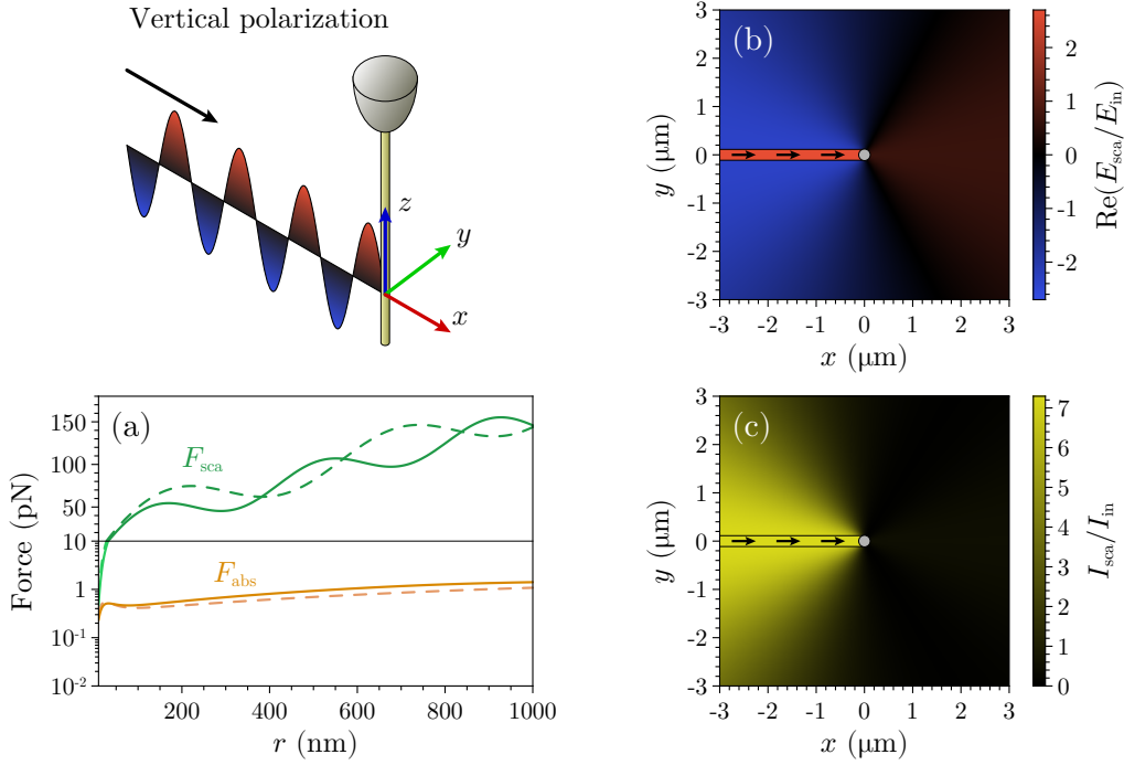
Figure 5.2: Scattering properties of a nanowire irradiated by a field with polarization parallel to the shaft. The nanowire is assumed to consist entirely of gold, with refractive index n_{\text{obj}} = 0.2 + 4.8i ( 0.2 + 7.0i ) for 780 nm (1064 nm) light. The refractive index of the medium, n_0 , is taken to be 1 regardless of whether the nanowire is in air or in vacuum. (a) Forces due to scattering (green) and absorption (orange) as a function of the radius of the nanowire, calculated according to Eq. 5.6–5.7. The traces are plotted for a beam of width W = 10 \mu\text{m} , power of 50 mW, and a wavelength of 780 nm (continuous) or 1064 nm (dashed). (b–c) Angular distribution of the scattered field and its intensity, as calculated from Eq. 5.1. The nanowire is placed at the origin and is assumed to have a radius of 120 nm. The incident light, of wavelength \lambda = 780 \text{ nm} , is approaching from the negative x axis. Its colour is adjusted to the maximum value of the scale rather than normalized to 1 in order to reveal the polarization at a glance.
