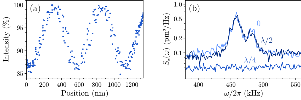
Figure 5.6: The output field of an optical cavity is influenced by the position of the nanowire within. The nanowire used is \approx 30\text{ }\mu\text{m} long, \approx 200\text{ nm} thick, gold-coated, and in air. (a) Variation of the intensity of the cavity's reflected field as a function of the nanowire's position. The intensity is scaled to the value at resonance when the nanowire is out of the cavity. (b) Detection of the nanowire's thermal fluctuations from the cavity output. When the nanowire is at an anti-node (lightest and darkest traces) the eigenmodes are detected thanks to the interaction with the cavity field. When the position is shifted to coincide with a node, no eigenmodes can be detected.
