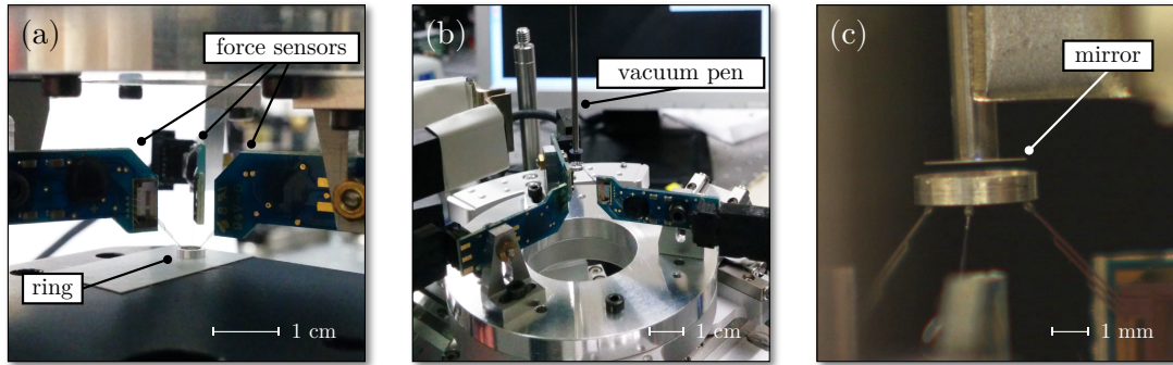
Figure 9.3: Different steps in the preparation of the stage for the upper mirror. (a) Attaching the supporting ring to the tips of the three force sensors. (b) Holding the mirror with the vacuum pick-up pen during positioning. (c) Close-up of the mirror held by the vacuum pick-up pen just before releasing it onto the ring.
