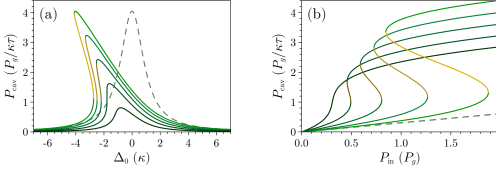
Figure 3.3: Effects of optomechanical bistability on the cavity. All the powers are normalized in terms of P_g := \hbar\omega_c |\alpha_s|^2 \big|_{G_0 x_s = \kappa} = \omega_c \kappa^2 m \omega_m^2 / g^2 . The parameters of interest have the following values: m = 1 kg, \omega_m = 2\pi \times 10 Hz, \omega_c \approx 2\pi \times 280 THz, \mathcal{F} = 1000 . (a) Intra-cavity power as a function of detuning. The traces, from darker to lighter, correspond to the power P_{\text{cav}} = \hbar\omega_c |\alpha_s|^2 at input power P_{\text{in}} between 0.2 and 1.0 P_g , at intervals of 0.2 P_g . (b) Intra-cavity power as a function of input power. Different traces now correspond to an increasingly more negative detuning \Delta_0 , ranging from -1.5 \kappa (darker) to -3.5 \kappa (lighter) at intervals of 0.5 \kappa . In both plots, in the presence of bistability, the unstable solution is represented in yellow. The dashed traces show what intra-cavity power would be obtained in the absence of optomechanical interaction at an input power P_{\text{in}} = P_g (a) or at a detuning \Delta_0 = -3.5 \kappa (b).
