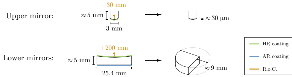
Figure 9.2: The cavity mirrors required special adjustments in order to be ready for the tripod. The upper mirror, originally about 5 mm thick, was lapped to a spherical cap of thickness of \approx 30 \mu\text{m} . The lower mirrors, with high-reflective coating on the concave side and anti-reflective coating on the flat side, had to be sliced so that their centres could be placed closer.
