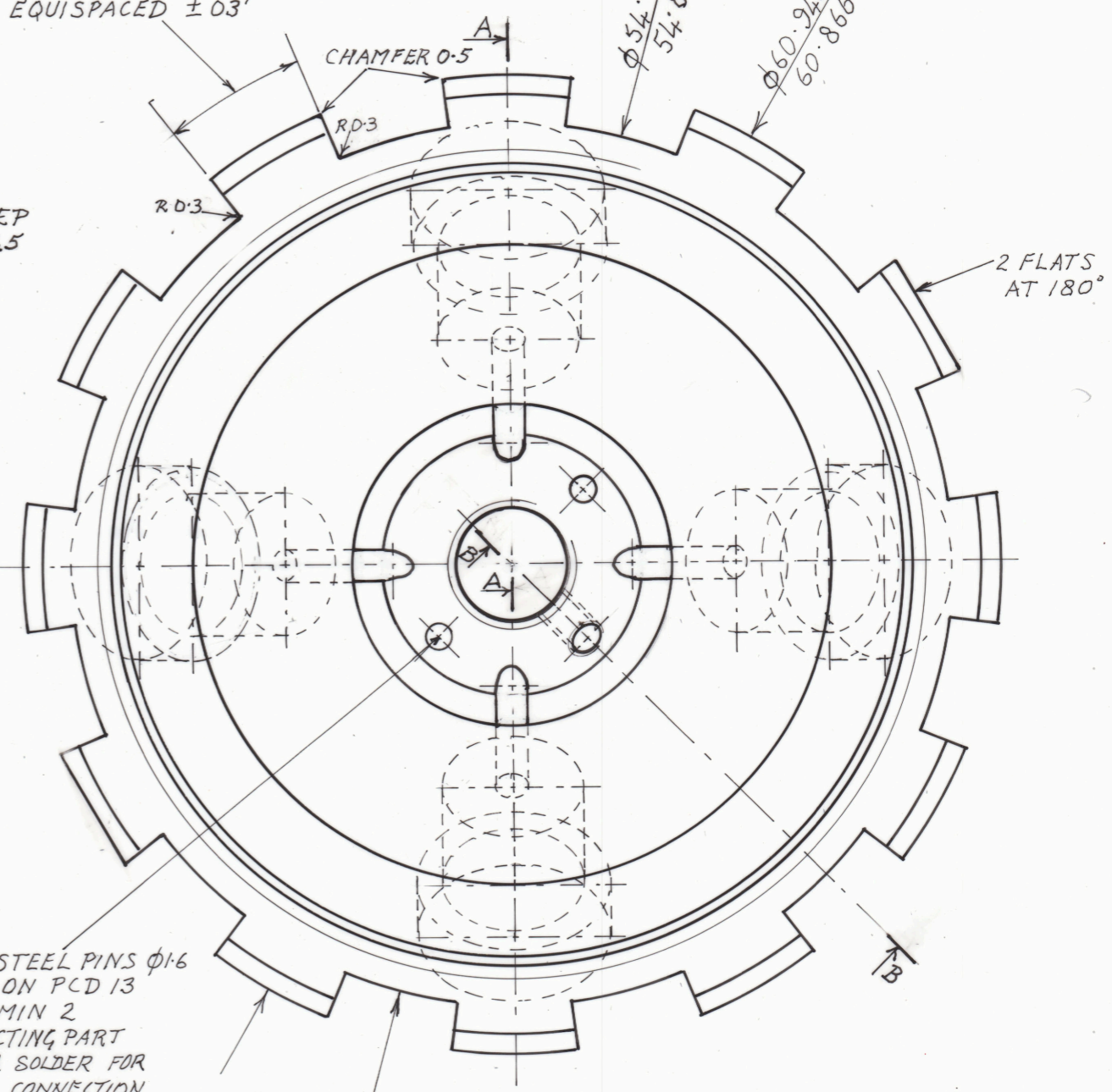
BOTTOM VIEW DRG 4302A
