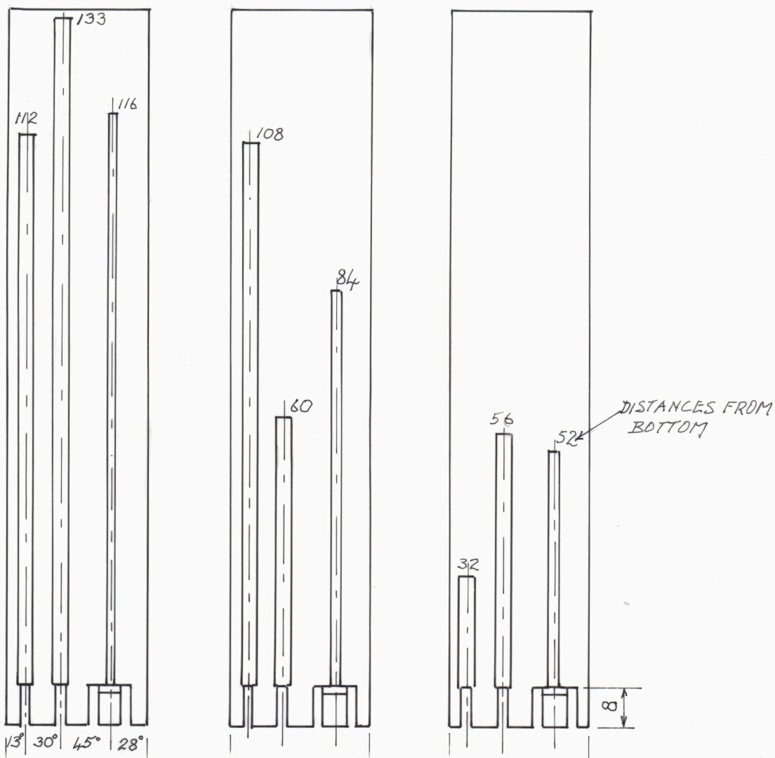
PROJECTION FROM CENTRE OF GROOVES FOR LEADS
