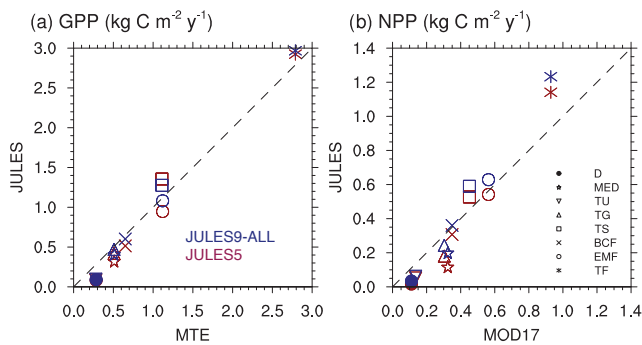
Figure 6. Annual GPP and NPP for the eight biomes shown in Fig. 3b. Biome abbreviations are D – deserts, M – Mediterranean woodlands, TU – tundra, TG – temperate grasslands, TS – tropical savannahs, BCF – boreal and coniferous forests, EMFs – extratropical mixed forests, TF – tropical forests.
