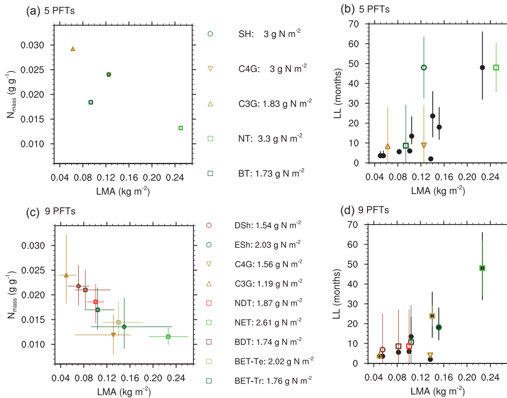
Figure 1. Trade-offs between leaf mass per unit area (LMA; kg\ m^{-2} ) and (a, c) leaf nitrogen ( g\ g^{-1} ), and between LMA and (b, d) leaf life span (LL). (a, b) Parameters in the standard JULES, converted from N_{l0} and \sigma_l based on 0.4\ kg\ C per kg dry mass (assumed parameter in JULES from Clark et al., 2011). (c, d) Median values from the TRY database for the new nine PFTs. In (b) and (d), the filled circles show the observed data and the open shapes show the median values from global simulations of JULES from 1982 to 2012. Vertical and horizontal lines show the range of values between the lower and upper quartile of data.
